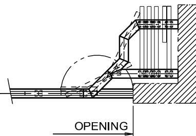
90° CRANK DOG LEG STACK WITH HALF HINGED ACCESS PANEL
