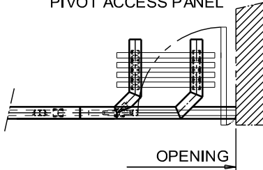
90° PARALLEL STACK WITH PIVOT ACCESS PANEL
