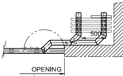
90° PARALLEL DOG LEG STACK WITH HALF HINGED ACCESS PANEL
