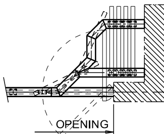
90° CRANK DOG LEG STACK WITH PIVOT ACCESS PANEL
