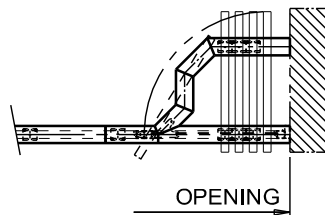
90° CRANK STACK WITH PIVOT ACCESS PANEL
