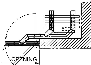
90° PARALLEL DOG LEG STACK WITH PIVOT ACCESS PANEL
