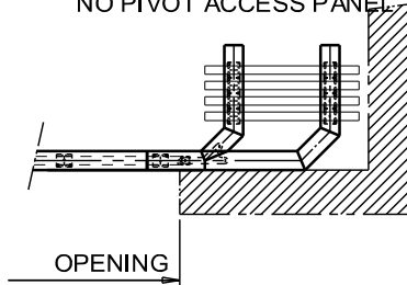
90° PARALLEL STACK WITH NO PIVOT ACCESS PANEL
